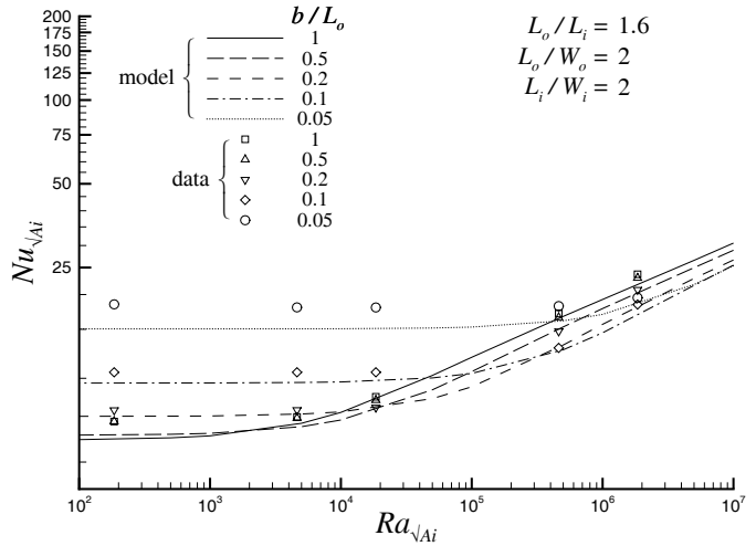
Fig. 15 Convection Model Validation: L/W = 2 , L_o/L_i = 1.6
