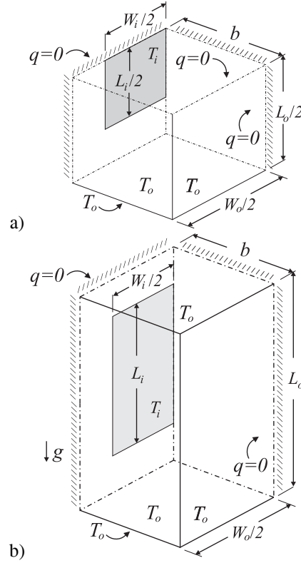
Fig. 4 CFD Model Solution Domains: a) Flotherm [13] Conduction Model; b) Icepak [14] Convection Model
