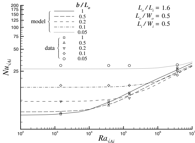
Fig. 13 Convection Model Validation: L/W = 0.5 , L_o/L_i = 1.6
