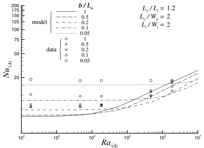
Fig. 14 Convection Model Validation: L/W = 2 , L_o/L_i = 1.2
