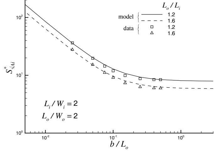
Fig. 8 Conduction Shape Factor Model Validation: L/W = 2
