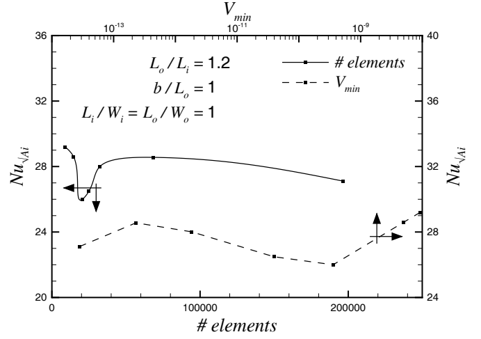
Fig. 6 Grid Convergence: Convection Simulations
