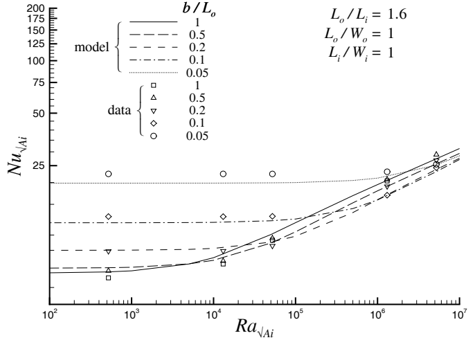
Fig. 11 Convection Model Validation: L/W = 1, L_o/L_i = 1.6
