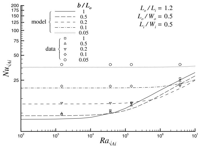
Fig. 12 Convection Model Validation: L/W = 0.5 , L_o/L_i = 1.2
