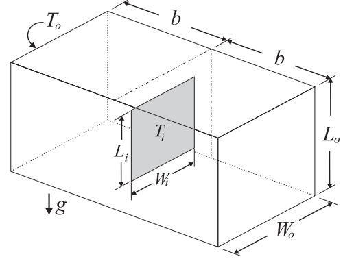
Fig. 1 Schematic of Enclosure Geometry
