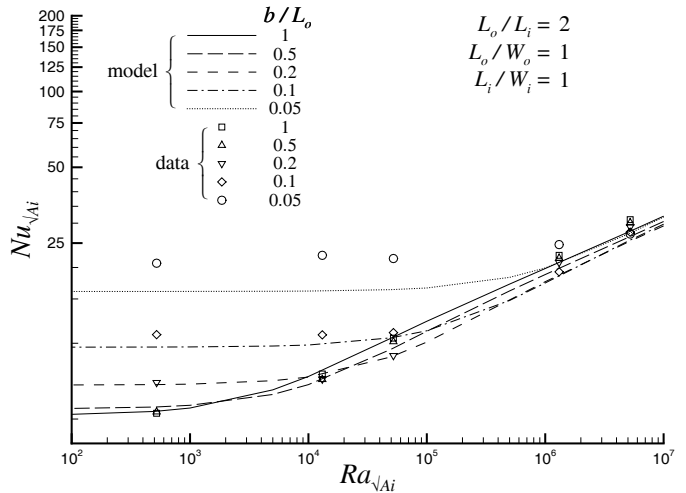
Fig. 12 Convection Model Validation: L/W = 1, L_o/L_i = 2.0
