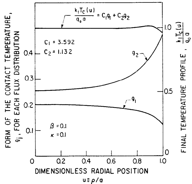
Fig. 4 Contact temperature rise for the Neumann solutions and their linear superposition: \beta = .1, \kappa = .1 .
