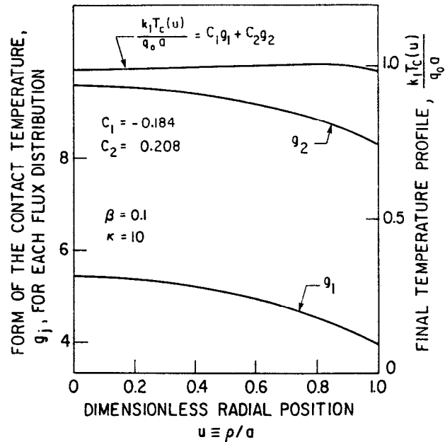
Fig. 5 Contact temperature rise for the Neumann solutions and their linear superpositions: \beta = .1, \kappa = 10 .
