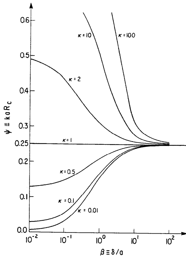
Fig. 6 Approximate isothermal constriction parameter, \psi_{ai} , versus the relative layer thickness conductivity ratio.
