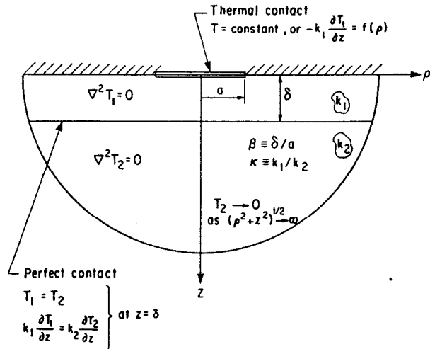
Fig. 3 Circular contact spot on a coated half-space.
