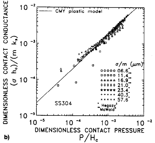
Fig. 4 Comparison of a) Mikic elastic model and b) CMY plastic model with SS304 data.
