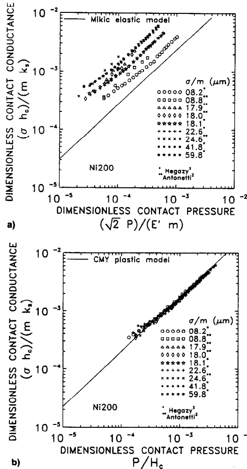
Fig. 3 Comparison of a) Mikic elastic model and b) CMY plastic model with Ni200 data.
